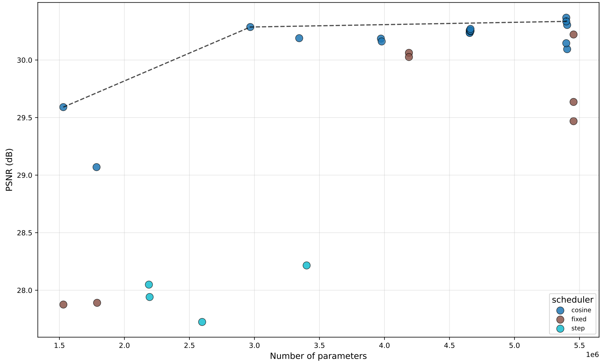
PSNR vs #Params — WaveletAttention — by scheduler
